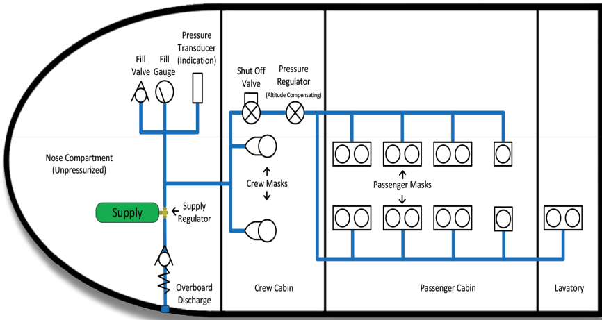
Typical PGOS System (Portable Gaseous Oxygen System)
